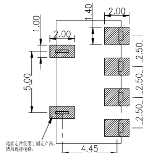
RECOMMENDED PCB LAYOUT TOP VIEW (.XX±0.05)
