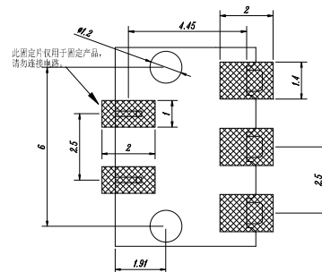
RECOMMENDED PCB LAYOUT TOP VIEW (. XX±0. 05)
