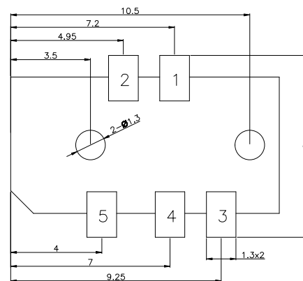
HOLE LAYOUT
