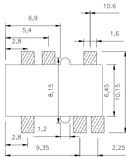
HOLE LAYOUT
