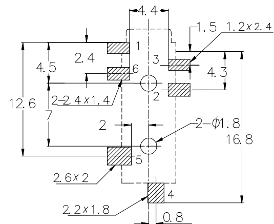
HOLE LAYOUT
