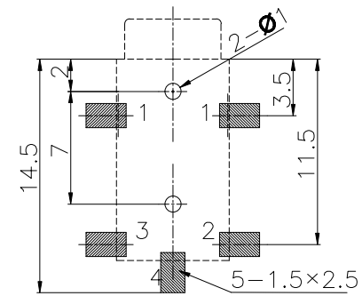
HOLE LAYOUT
