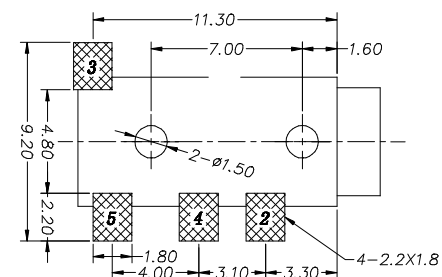
HOLE LAYOUT
