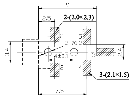
HOLE LAYOUT
