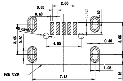
RECOMMENDED PCB LAYOUT (TOL: \pm 0.05 )
