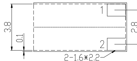
PCB LAYOUT TOP VIEW
