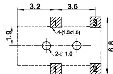
HOLE LAYOUT
