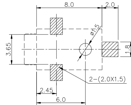
HOLE LAYOUT
