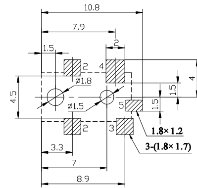
HOLE LAYOUT
