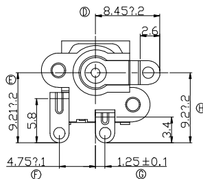
MATE PLUG
