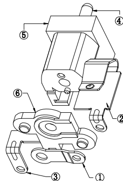
MATE PLUG
