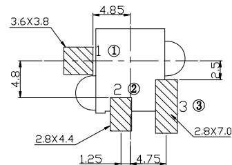
HOLE LAYOUT
